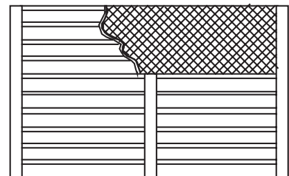
C. Spaced board panel with 1\frac{1}{2} -inch air gaps between boards. Panel may be totally solid (shown on left) or with stall guard (wire mesh shown on right). Center wall board support is needed.
